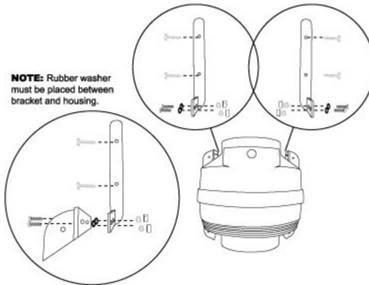
FIGURE 1: MOUNTING BRACKETS
