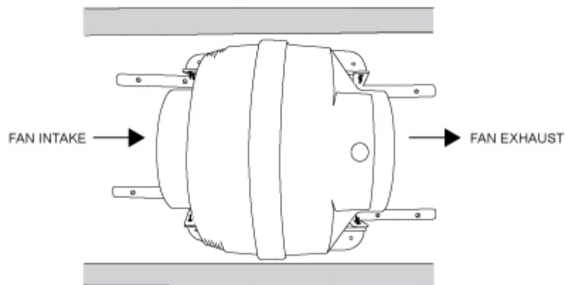
FIGURE 2: MOUNTING
