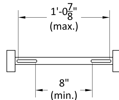
Spacer Bar Detail (Showing Range of Bolt Spacing)
