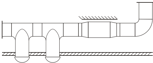
Figure 2. Installing / Instalación / Installation: TD - SILENT SERIES.
